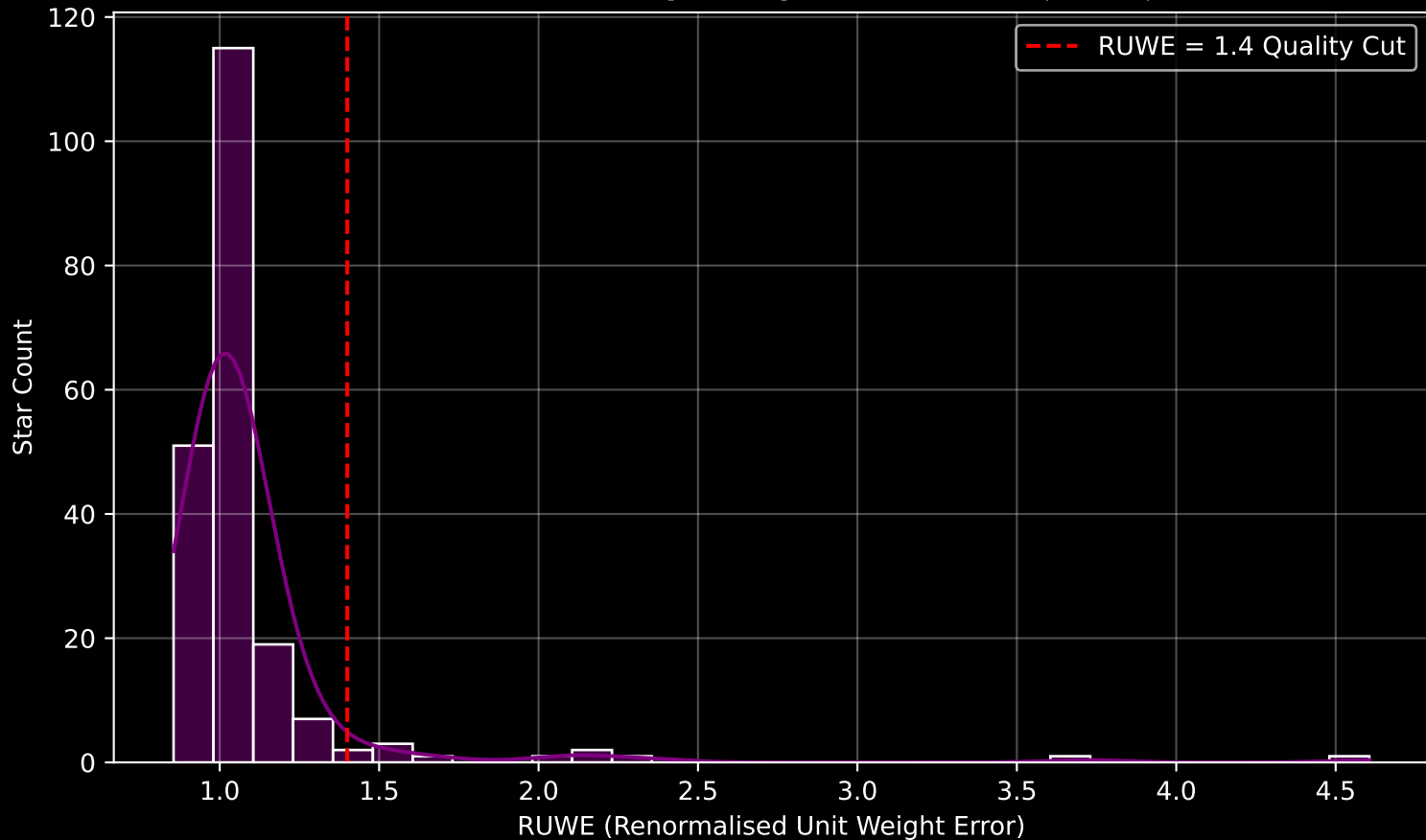
GAPOGEE DR17 Field [117+01] RUWE Distribution (n= 204)
