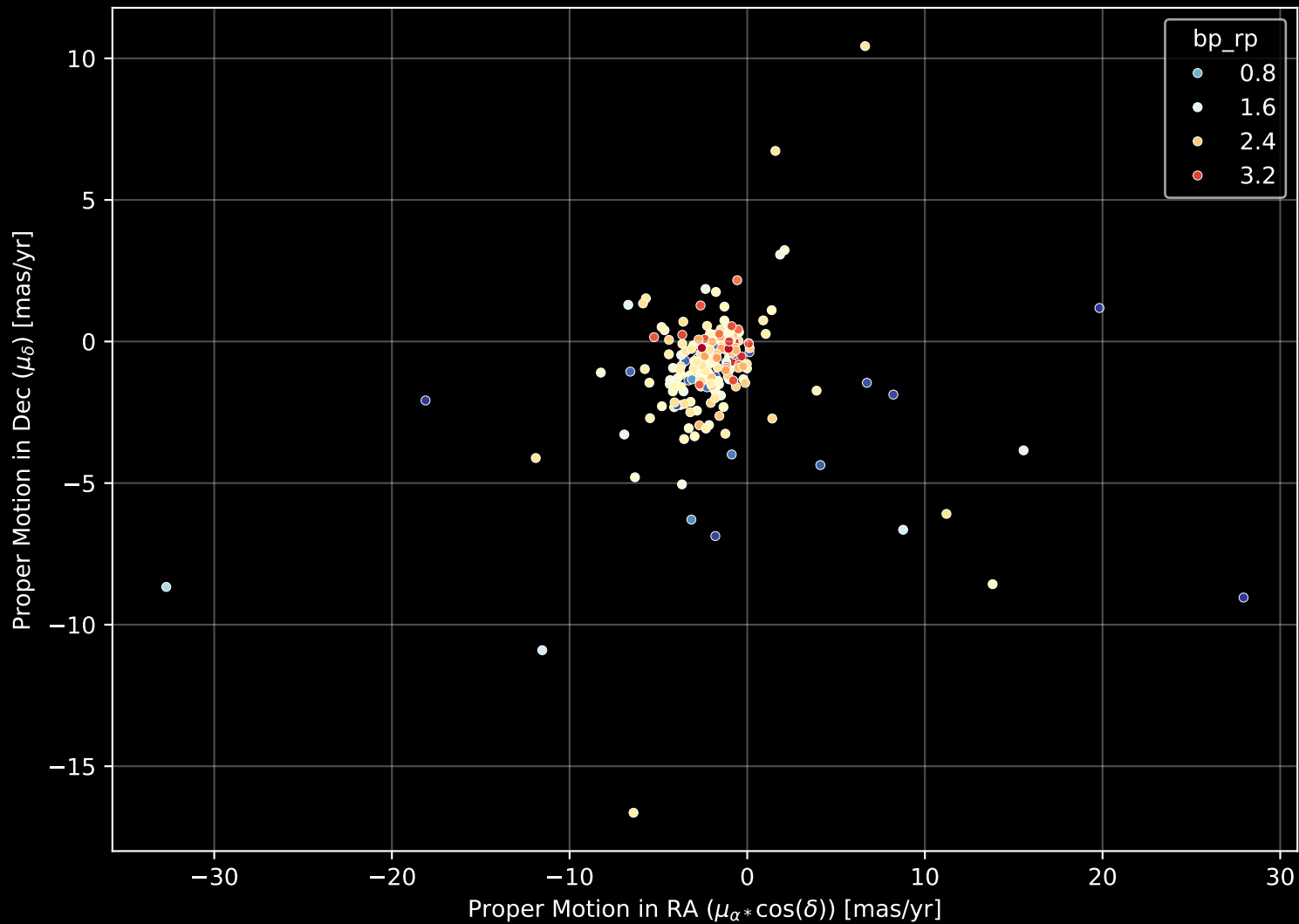
APOGEE DR17 Field: [117+01] Proper Motion Diagram (n= 210)
