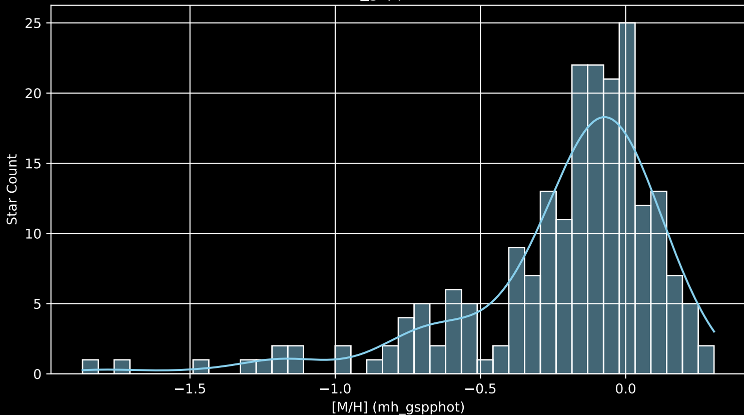
APOGEE DR17 Field: [117+01 [M/H] (mh_gspphot) (n= 208)
