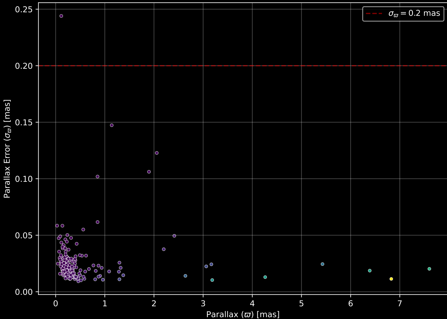
APOGEE DR17 Field: [117+01] Parallax Quality (n= 210)
