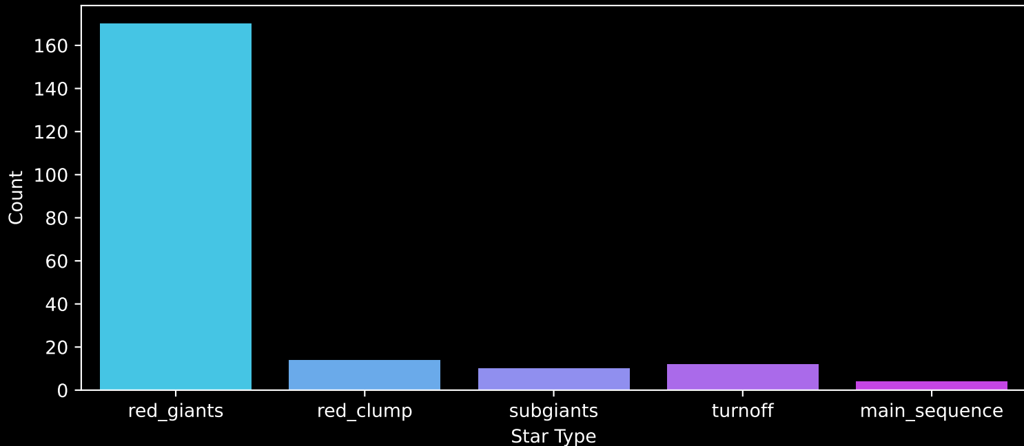
APOGEE DR17 Field: [117+01] Count plot of Star Type
